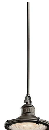
42436OZ | Sayre™ (1) 60W, Medium, 10"W x 8.5"H Overall Ht. 47", Chain / Stem 36"
